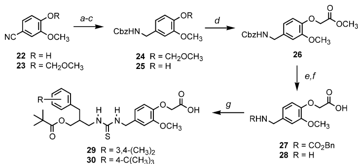
Scheme 3. Reagents: (a) ClCH 2 OCH 3 , NEt( i -Pr) 2 , CH 2 Cl 2 ; (b) (i) LiAlH 4 , THF; (ii) BnOCOCl, NEt 3 , CH 2 Cl 2 ; (c) CF 3 CO 2 H, CH 2 Cl 2 ; (d) BrCH 2 CO 2 CH 3 , K 2 CO 3 , acetone; (e) NaOH, THF–H 2 O; (f) H 2 , Pd/C MeOH; (g) 2-(3,4-dimethyl(or 4- t -butyl)benzyl)-3-pivaloyloxypropylisothiocyanate, NEt 3 , DMF.
