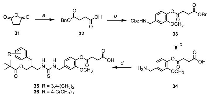
Scheme 4. Reagents: (a) BnOH, NaH, THF; (b) 25 , DCC, DMAP, CH 2 Cl 2 ; (c) H 2 , Pd/C, MeOH; (d) 2-(3,4-dimethyl(or 4- t -butyl)benzyl)-3-pivaloyloxypropylisothiocyanate, DMF.
