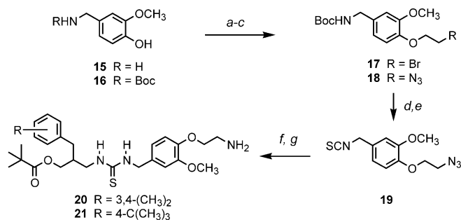
Scheme 2. Reagents: (a) Boc 2 O, NEt 3 , dioxane–H 2 O; (b) BrCH 2 CH 2 Br, KOH, Bu 4 NOH; (c) NaN 3 , DMF; (d) CF 3 CO 2 H, CH 2 Cl 2 ; (e) 1,1-thiocarbonyl di-2(1H)-pyridone, NEt 3 , DMF; (f) (i) 4 (or 5 ), H 2 , 5% Pd/C, MeOH; (ii) CH 2 Cl 2 ; (g) PPh 3 , H 2 O–THF.
