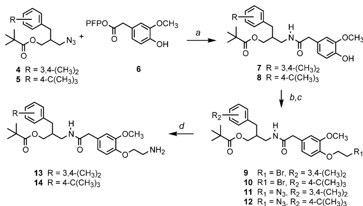
Scheme 1. Reagents: (a) (i) H 2 , Lindler's cat, EtOH; (ii) 6 , EtOAc; (b) BrCH 2 CH 2 Br, KOH, Bu 4 NOH; (c) NaN 3 , DMF; (d) H 2 , Pd/C, MeOH.
